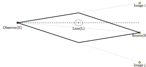
Figure 2.36: Configuration of a strong gravitational lensing system. The thick solid line shows the two different paths that photons emitted from the source could take. The dotted lines show the angular positions where images and the source appear on the sky. The position of the source, however, is usually not observable as it is very close to the lens. Note that the plot is not to scale: The distance photons travel is much longer than the size of the lens or the source. Credit: Jee, Komatsu and Suyu 2014
