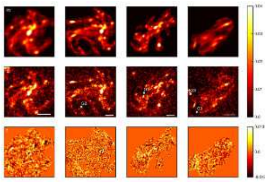
Figure 2.28: Results for the surface brightness modelling of the multiply imaged face-on galaxy. Images from left to right are the main images 1.1, 1.2, 1.3.1 and 1.3.2. The top row shows the model reconstruction, the middle row the observed data and the bottom row the residual (i.e. the difference between model and data).
