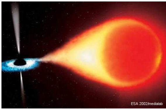
Figure 2.23: An artist's impression of an accreting Low Mass X-ray Binary. The donor star fills its Roche lobe and its material overflows the inner Lagrangian points and accretes on the relativistic star (in this case a black hole). Due to the large angular momentum of the infalling material an accretion disk is formed around the compact object. Credit: ESA 2002/medialab
