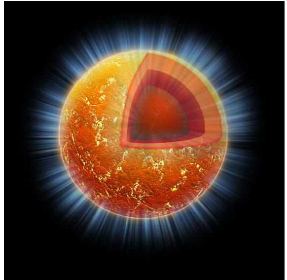
Figure 2.2: Neutron star structure: A solid crust with a thickness of about 1km surrounds a liquid core of about 10km whose state of matter is largely unknown. Credit: Illustration of Cassiopeia A: NASA/CXC/M.Weiss
