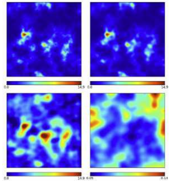
Figure 2.15: A simulated observation of a galaxy cluster with the VLA. The image on the top left shows the (real) input signal. The top right image shows the reconstruction using the RESOLVE algorithm. The image on the bottom left shows a reconstruction with a standard algorithm (CLEAN) while the image on the bottom right gives the relative uncertainty of the reconstruction, note the different scale on this map.
